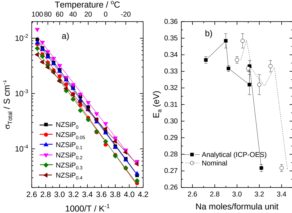
Fig. 7: a) The Arrhenius plot of \sigma_{\text{total}} obtained from impedance spectroscopy in the temperature range -30 – 100 °C and b) the E_a as a function of nominal and analytical composition.
