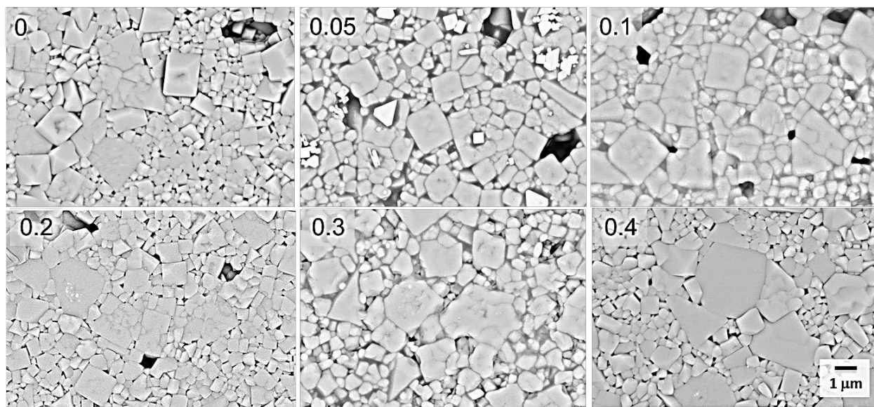
Fig. 5: Microstructure of \text{Na}_{3+x}\text{Zr}_2\text{Si}_2\text{PO}_{12+x/2} ceramics obtained after two-step sintering and thermal etching at 1150 °C for 0.25 h.
